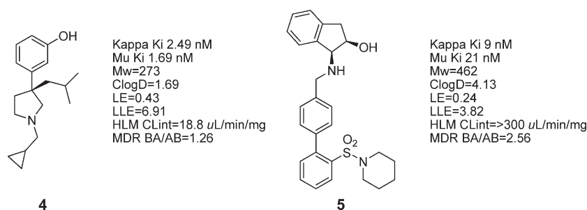
Figure 2. HTS lead structures 4 and 5.
