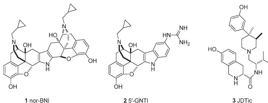
Figure 1. Structures of nor-BNI (1), 5'-GNTI (2), and JDTic (3).
